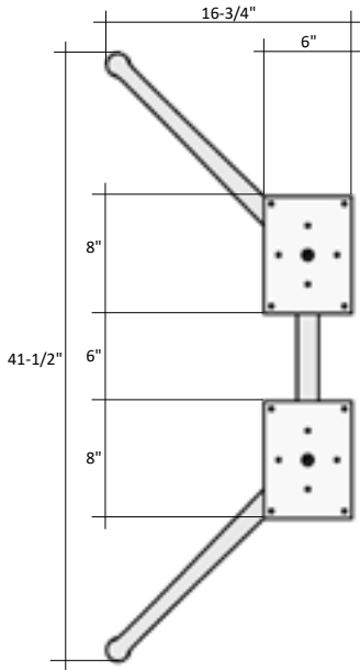
For 54" and 60" Deep Table Tops
