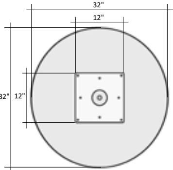
For 48" Round or 42" Square Table Tops
