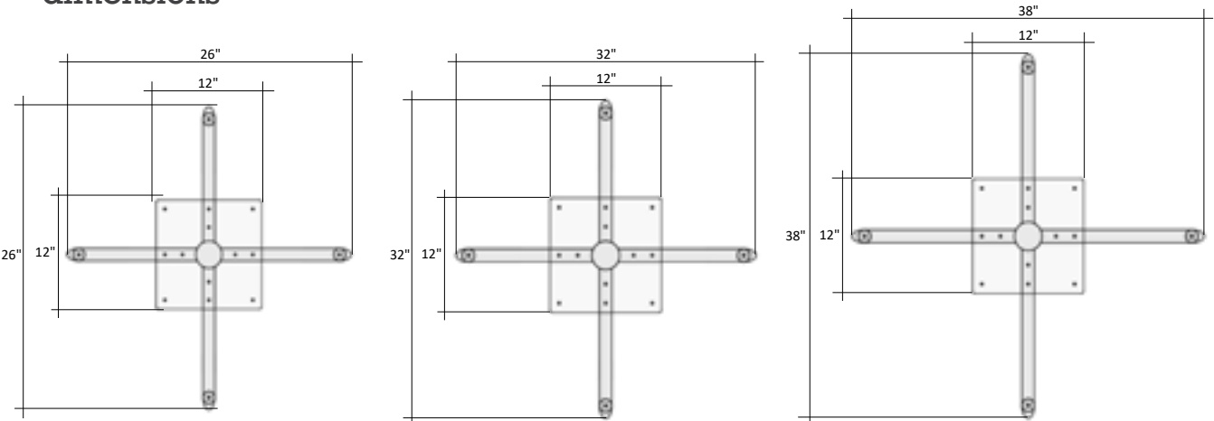
For 30" and 36" Round and 30" Square Table Tops
