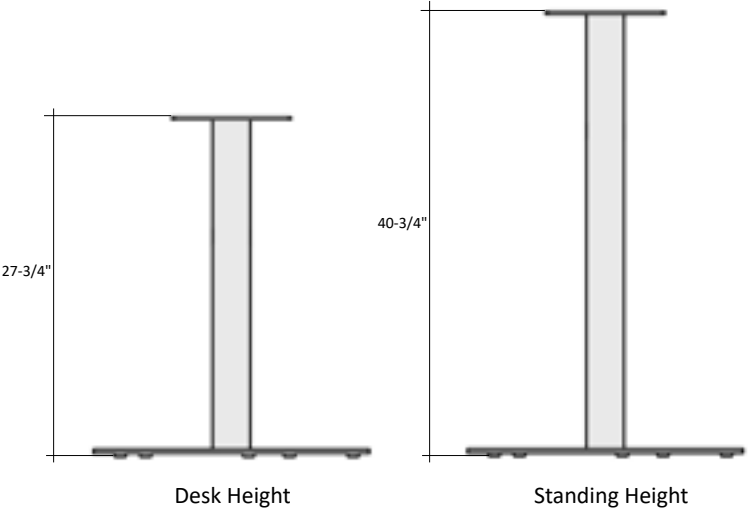
For 30" and 36" Round or 30" Square Table Tops
