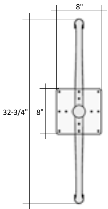
For 42" Deep Table Tops
