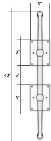
For 54" and 60" Deep Table Tops
