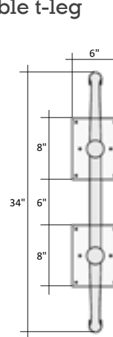
For 48" Deep Table Tops
