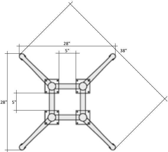
For 54" and 60" Round and 48" Square Table Tops
